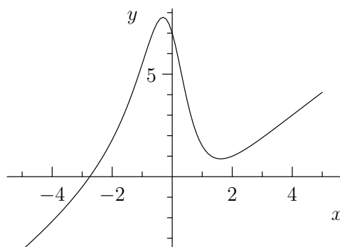
FIGURE IX2 – Graphe de x \mapsto \frac{x^3 - 5x + 7}{x^2 + 1}
